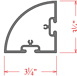
325/4000 Rad. Corner Post C7K3288
