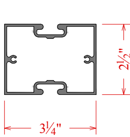
325 Dbl. Slot Post C7K8288
