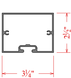
325 Std. Post C7K0288
