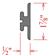
Center Mount Bracket C51522146
