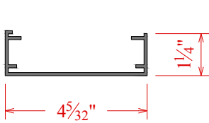
Univ. Raceway C51570146
