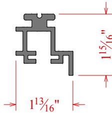
3000 Side Frame C6P30240
