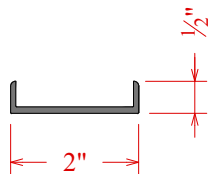
225 Radius Channel C6G04153
