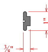
Stop Block/Post Filler C51523153
