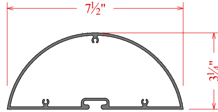
750 Rad. Post C7L2288
