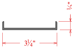
325 Radius Channel C6K04153
