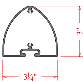
325 Contour Post C7I9240
