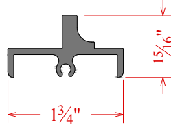
Dovetail Bottom w/ Screw Boss C51545153 (For Use in 8" or smaller CWBs, Order w/ C51541153)
