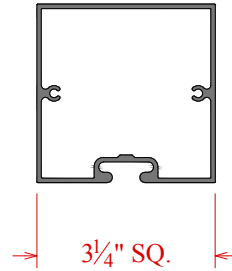
325 Sq. Post C7K92288
