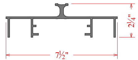
750 Flush Face Side Frame C6L10153
