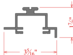
4000 Side Frame C6Q40146
