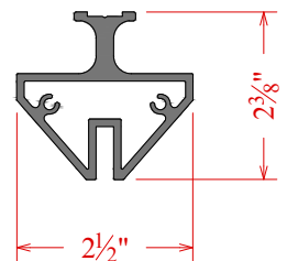
250 Side Frame C6H00153
