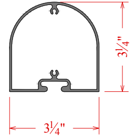
325 Ext. Rad. Post C7K4288
