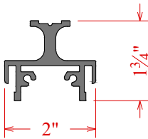
225 Std Side Frame C6G00153
