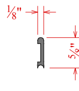
5/8" Graphic Bar C51550050
