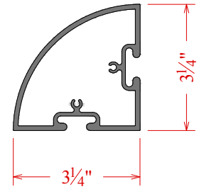
325/4000 Rad. Corner Post C7K3288
