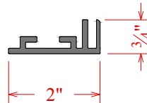
3000 T/B Frame C6P31240
