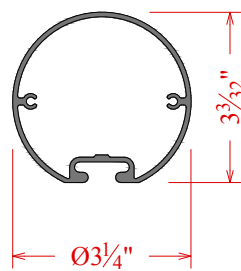
325 Full Rd. Post C7K5288
