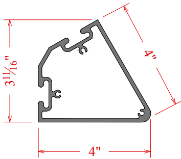
3000 Triangular Post C7P0240
