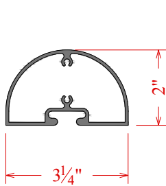
325 Rad. Post C7K2288
