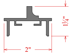
Dovetail Bottom w/ Corner Key Slot C51542153 (For Use CWBs over 8", Order w/ C51541153)
