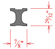
Univ. Dovetail C51544146
