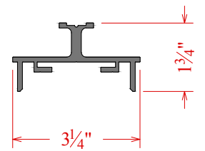
325 Flush Face Side Frame C6K10153
