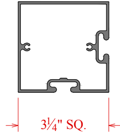
325/4000 Corner Post C7K6288
