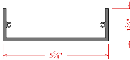
Base Mount Channel, Bottom C51576218
