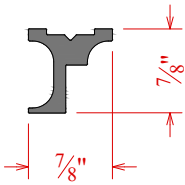
Dovetail Top C51541153 (Order w/ C51542153 or C51545153)
