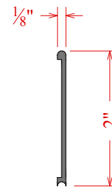
2" Graphic Bar C51552146
