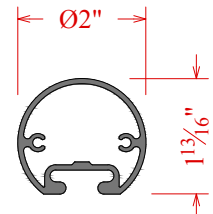
225 Full Rd. Post C7G5288
