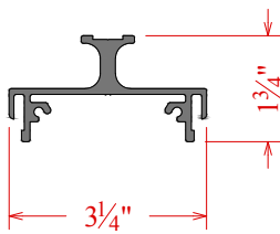
325 Std. Side Frame C6K00153
