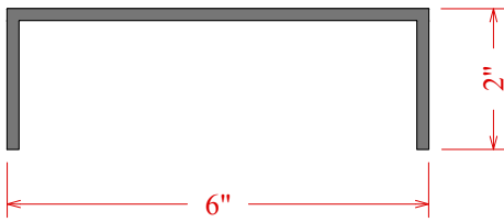
Base Mount Channel, Top C51575218
