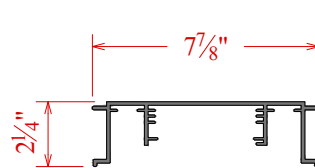
1200 Base Frame C6M51219 (Order w/ C6M53219)
