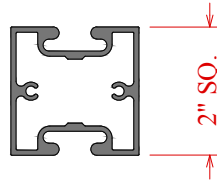
225 Dbl. Slot Post C7G8288
