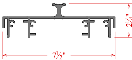
750 Std. Side Frame C6L00153
