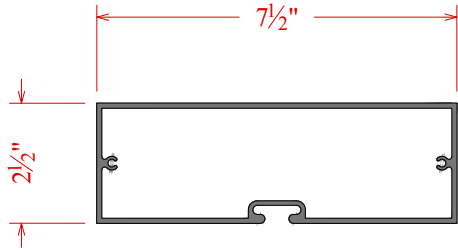
750 Std. Post C7L0288
