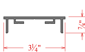
325 Flush Face T/B Frame C6K11153
