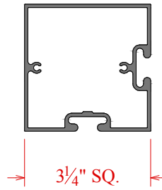
325/4000 Corner Post C7K6288
