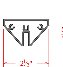
250 Std. Frame/Econo Post C7J1192
